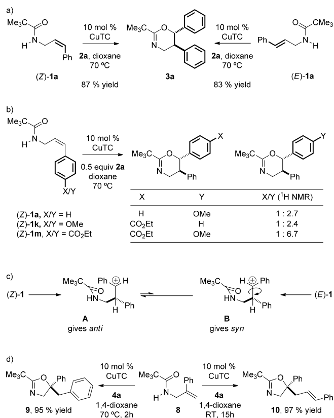
Scheme 5. Mechanistic investigations. a) The effect of alkene geometry. b) Competition experiments to investigate the effect of the electronic properties of the alkene. One equivalent of a 1:1 mixture of two allylic amides were treated with 2a under the standard reaction conditions. c) A possible carbocation mechanism. d) Location of cation-stabilizing groups can affect the selectivity of the cyclization.
