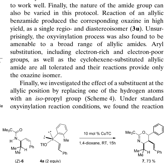
Scheme 4. Diastereoselectivity in the Cu-catalyzed oxyvinilation.
