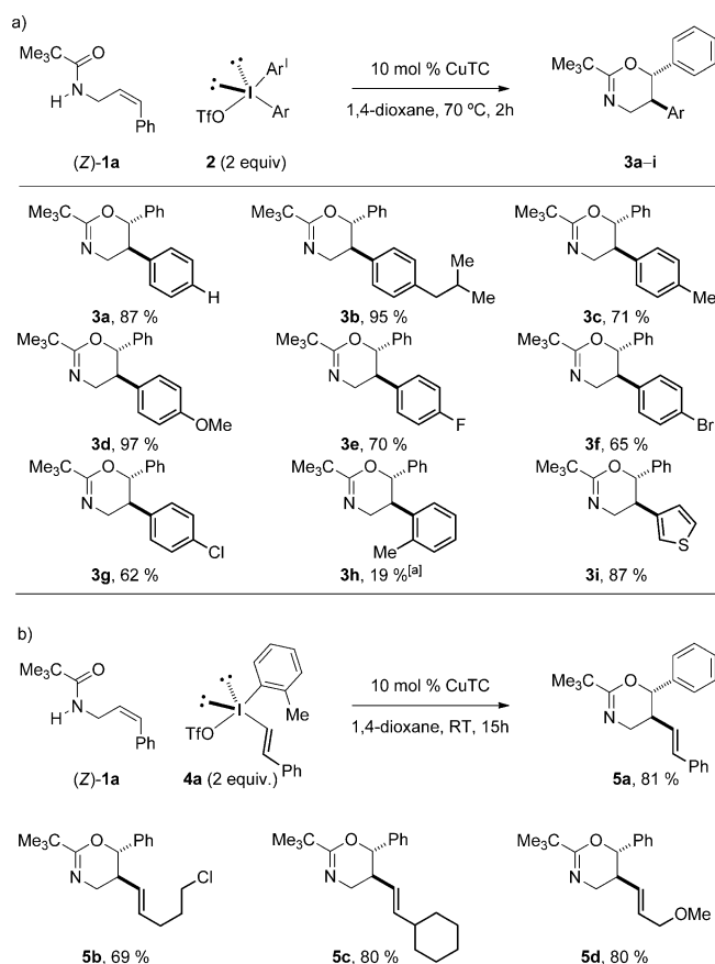
Scheme 2. Cu-catalyzed oxyarylation (a) and oxyvinylation (b) of allylic amides. [a] Yield determined by 1 H NMR spectroscopy with 1,3,5-(MeO 2 C) 3 C 6 H 3 as internal standard.
