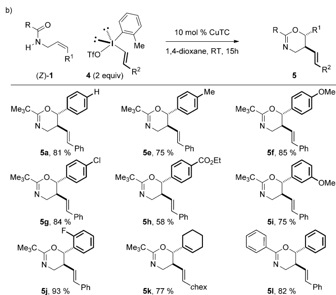
Scheme 3. Scope of alkene substituent in oxyarylation (a) and oxyvinilation (b).
